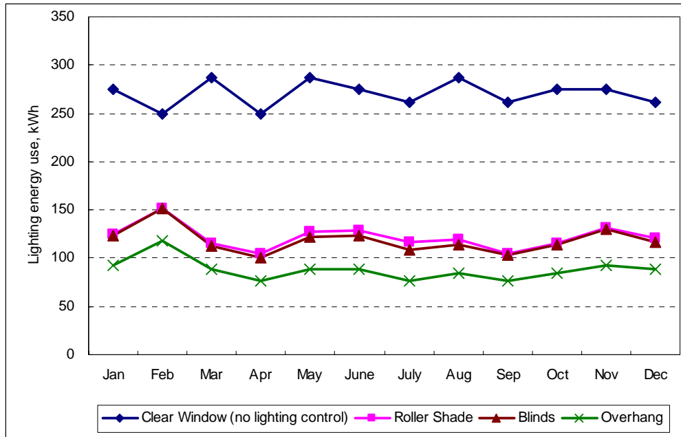
Fig. 12: Monthly lighting energy use in kWh for double clear low-e glazing
