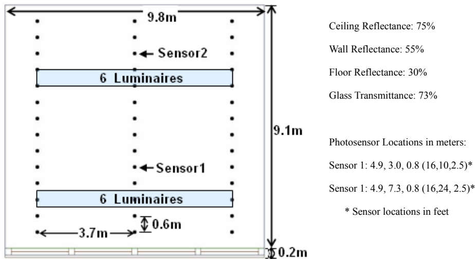
(a) Plan view with luminaires
