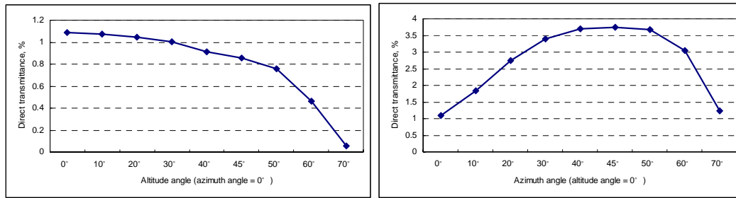
Fig. 6: Direct transmittance as a function of incident angle
