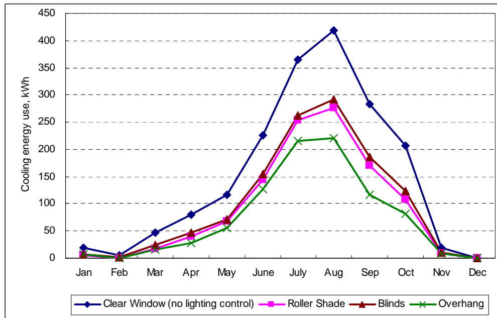
Fig. 13: Monthly cooling energy use in kWh for double clear low-e glazing
