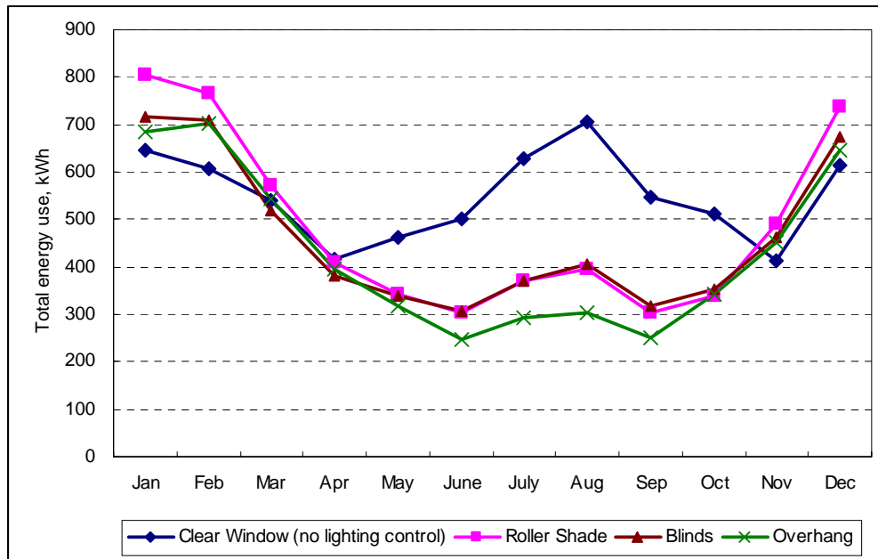
Fig. 15: Monthly total energy use in kWh for double clear low-e glazing
