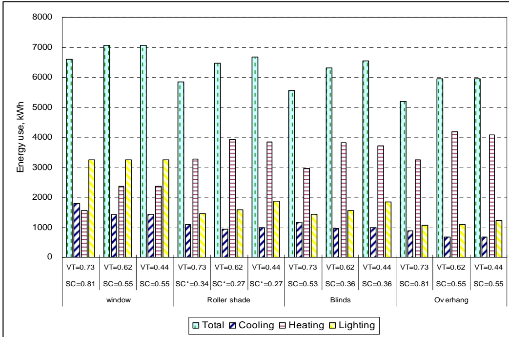
Fig. 16: Comparison of annual energy consumption for double clear, green, and bronze low-e glazings
