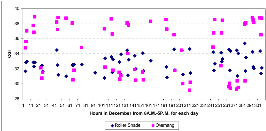
Fig. 18: CIE glare index comparison for shade and overhang for December
