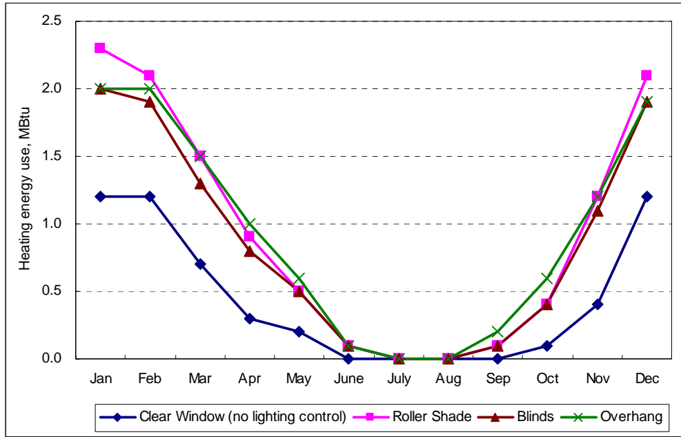
Fig. 14: Monthly heating energy use in MBtu for double clear low-e glazing
