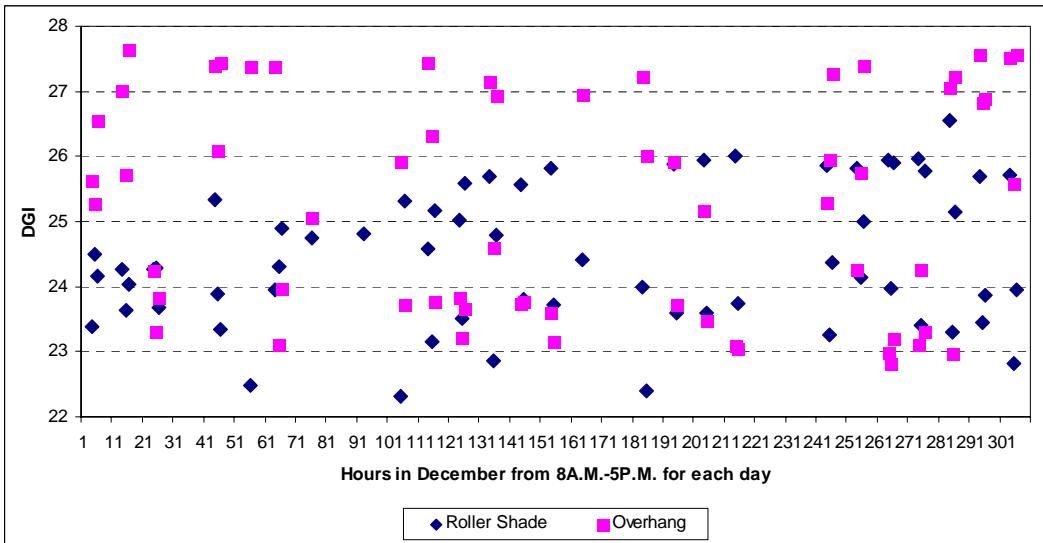
Fig. 17: Daylight glare index comparison for shade and overhang for December
