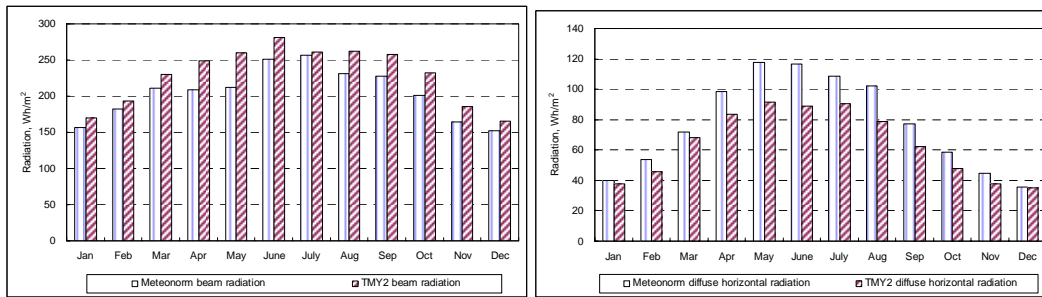
Fig. 10: Beam and diffuse horizontal radiation for Meteororm and TMY2
