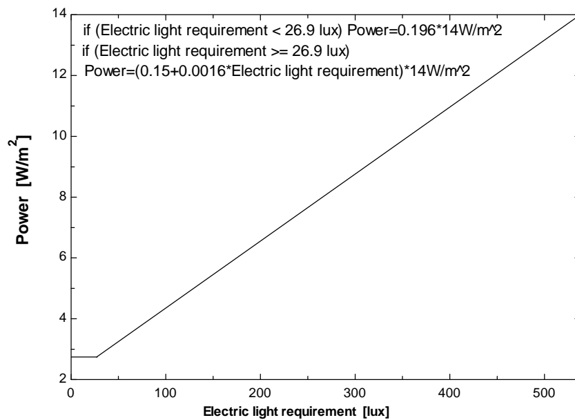
Fig. 11: Electric light dimming curve
