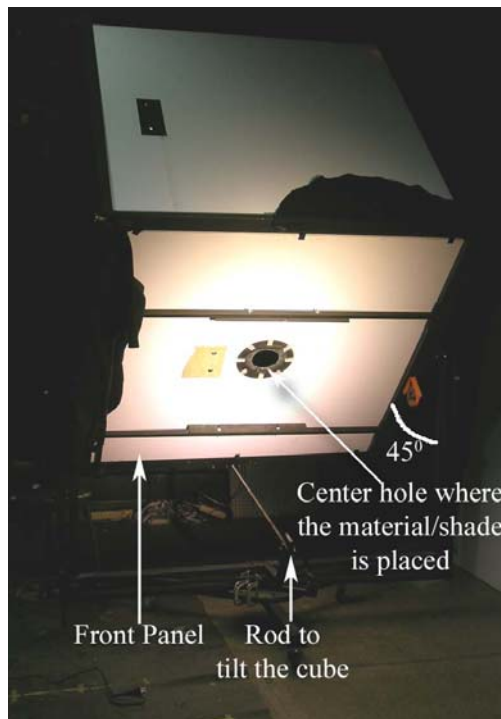
Fig. 2: The cube used for BTDF measurements
