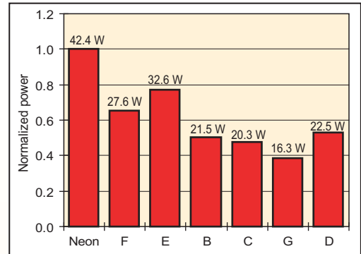
Comparison of all LED signs for equal light output of neon (red, above) and cold-cathode (CC) fluorescent (white, below) signs.
