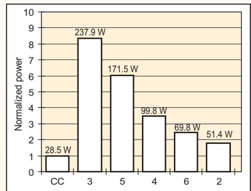
Comparison of all LED signs for equal light output of neon (red, above) and cold-cathode (CC) fluorescent (white, below) signs.
