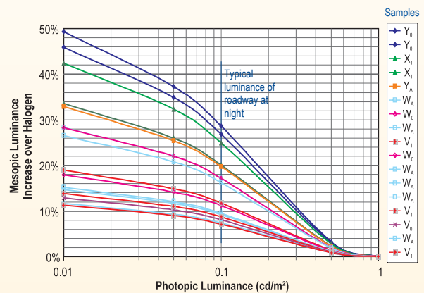
Increase in mesopic luminance of white LED test samples over a halogen headlamp source
