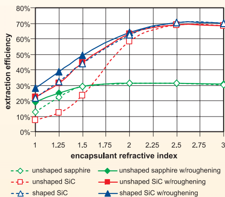
Extraction efficiency for three chips as a function of encapsulant refractive index with and without top surface roughening.
