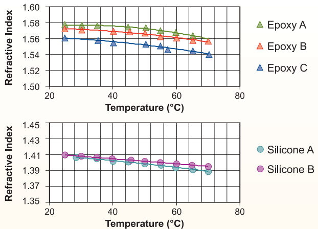
Refractive index change as a function of temperature of several commercial epoxies and silicone materials commonly used as LED encapsulants.
