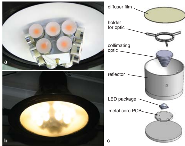
(a) The snap-in SPE LED modules in the luminaire housing; (b) the final prototype outdoor luminaire; (c) the snap-in module components.
