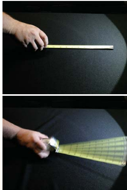
The photographs above were taken under a flickering light source (at 120 Hz) with an exposure time of 1/15th of a second. In the top photo, the ruler is stationary and no stroboscopic effects are seen. In the bottom photo, multiple images are produced by each flicker cycle as the ruler moves across the scene.
