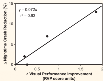
Provisional transfer function between visual performance improvements and observed nighttime crash reductions associated with roadway lighting at different intersection types.
